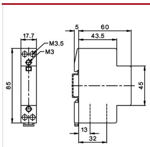
OptiDin MK63-40 OptiDin MK63-63
